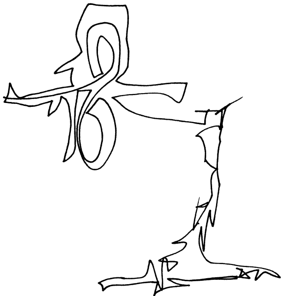
stress tree
